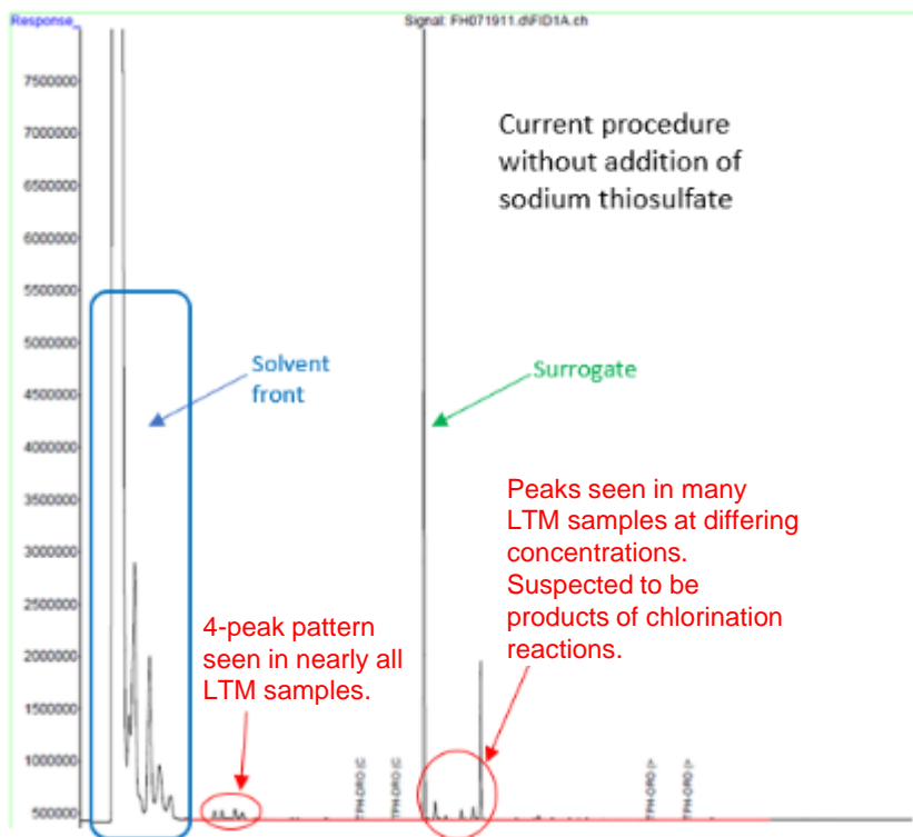
Figure C-1. Effect of Sodium Thiosulfate Addition (Quenching) Sample H3-TW-0013887-23335-A
